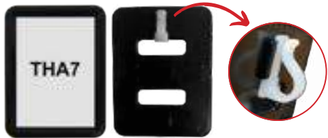
A7 Mini Frame Kit - (9 up) Frame, rear hook, PVC sheet 82 x 110 x 6mm THA7
